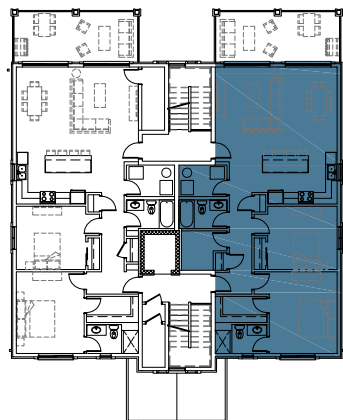
THIRD FLOOR
